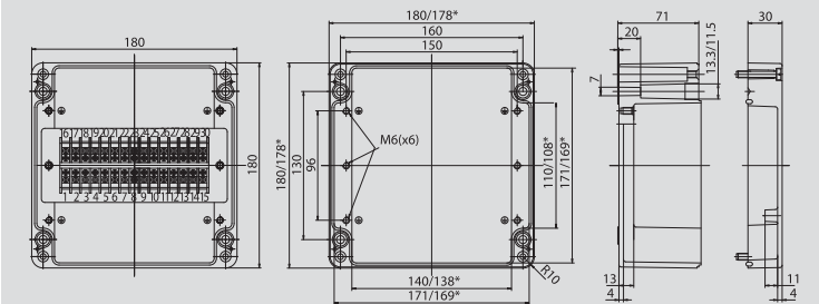
Dimension (허용오차 allowance ±1mm)
